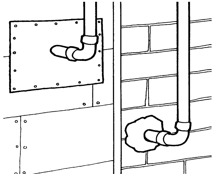
Figure 4. Rodentproofing openings around pipes with sheetmetal (left) and concrete (right).
