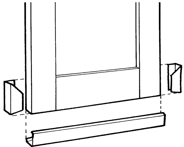
Figure 5. Rodentproofing a door, placing channel at bottom and cuffs at sides over channel.
